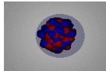
Pygmy resonance
