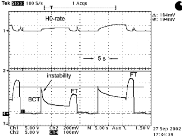
Fig. 6. In the first cycle, without sextupole, a strong beam loss after injection due to a coherent vertical betatron oscillations (instability) is visible in the beam current signal (BCT). This beam loss is compensated by the sextupole family in the next cycle. The flat top (FT) intensity is doubled. The horizontal line in the lower trace points at the same number of injected protons in both cycles. (100 mV BCT signal corresponds to 1 mA proton current).
