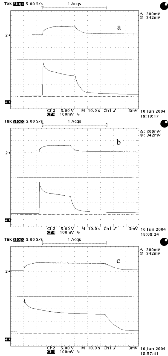
Fig. 10. Ion current versus time: a) shaker is off, b) non resonant excitation, c) excitation on resonant frequency of 114 kHz.
