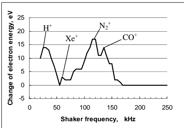
Fig. 8. Spectrum of resonance shaker frequencies measured at COSY cooler.
