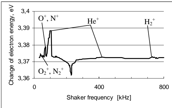
Fig. 7. Spectrum of resonance shaker frequencies measured at HIMAC cooler.
