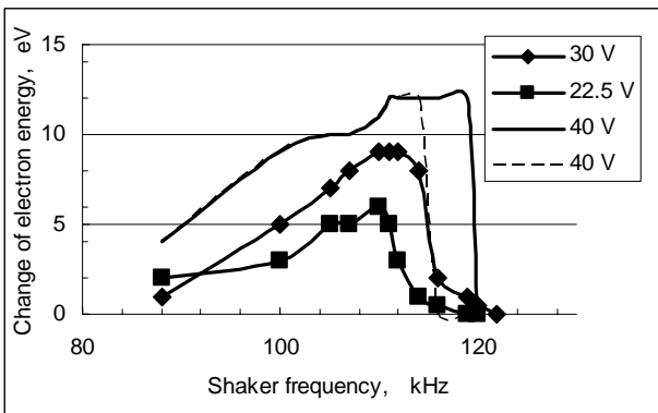
Fig. 9. Shape of the resonant peak at 90 – 120 kHz as function of the shaker voltage amplitude. At 40 V there is a hysteresis effect – solid line corresponds to an increase of the shaker frequency, dashed line – to a decrease.
