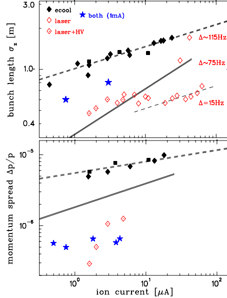
Figure 1: Spatial bunch length (pick-up) and momentum spread (Schottky signal and fluorescence diagnostics) for electron- and laser-cooled ion beams of decreasing current.
