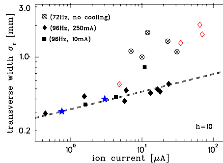
Figure 2: Transverse width (beam-profile-monitor) as above ( \sigma_r = 0.4 \text{ mm} corresponds to \varepsilon = 4 \times 10^{-3} \pi \text{ mm mrad} ).
