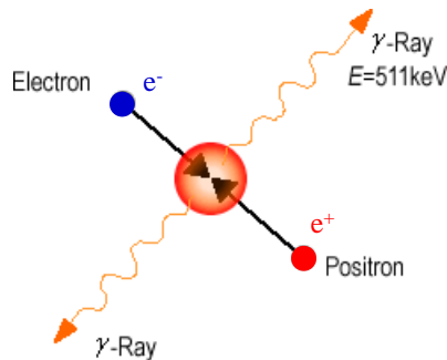
particle – anti-particle annihilation
